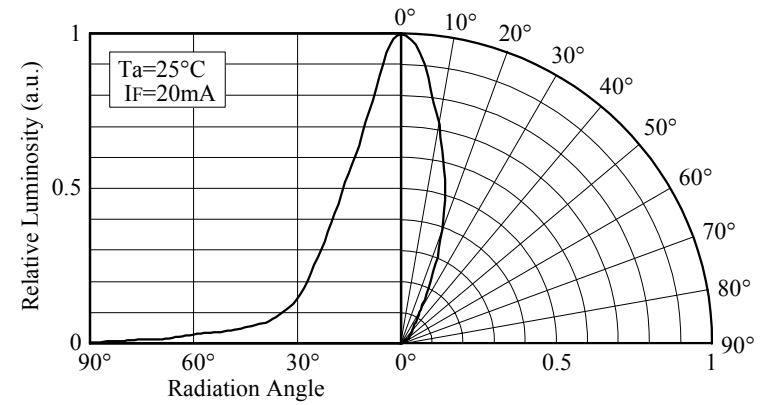
■ Directivity (NSPB310A)
