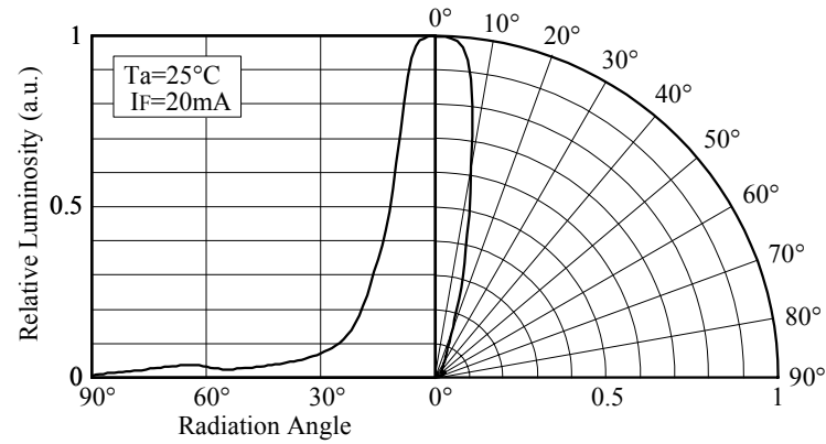
■ Directivity (NSPW300BS)
