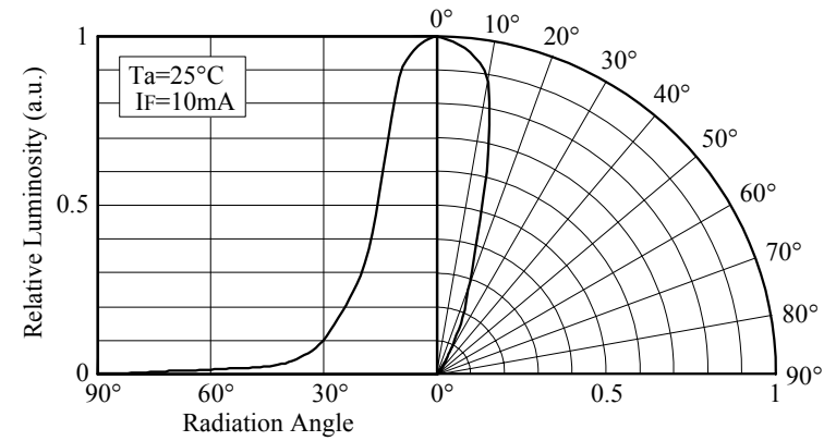
■ Directivity (NSPE510(S))
